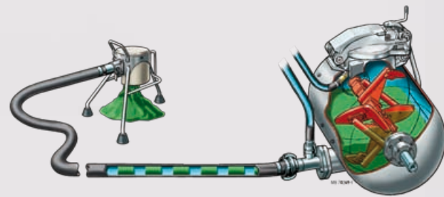
schematic diagram of the Mixokret pumping system
